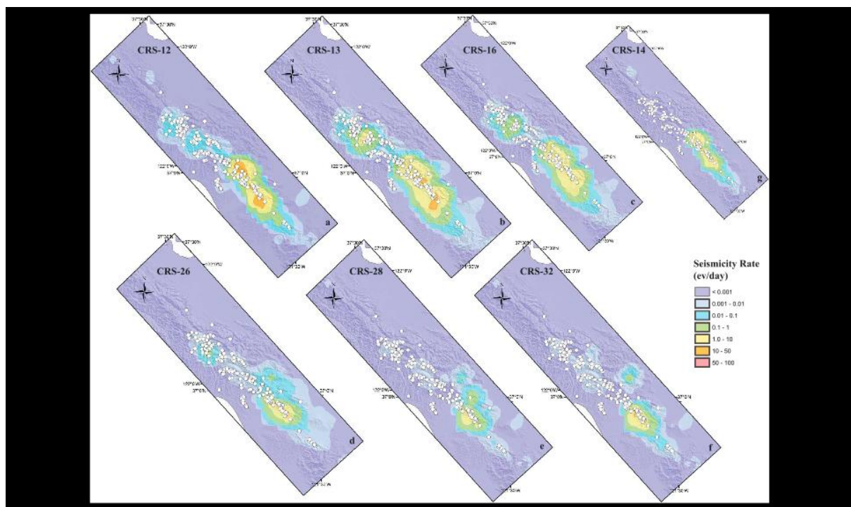
Figure 1: Maps of daily seismicity rates forecast by physics-based models (Segou et al., 2013) for the first 10 days after the magnitude 6.9 1989 Loma Prieta mainshock in Northern California for models based on (a) optimally oriented strike slip fault planes with a low-stressing rate San Andreas Fault (SAF) and a gridded reference seismicity model, (b) same as (a) but considering a smoothed gridded reference seismicity model, (c) same as (b) but considering a medium-stressing rate SAF, (d) receiver planes derived from predominant geology with a low-stressing rate SAF and a smoothed-gridded reference seismicity model, (e) receiver planes derived from predominant geology with a high-stressing rate SAF and a gridded reference seismicity model, (f) shear stress changes on receiver planes derived from predominant geology with a medium-stressing rate SAF and a smoothed-gridded reference seismicity model, and (g) same as (c) considering a declustered background seismicity model.
