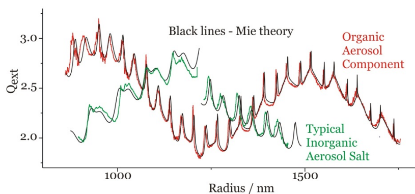
Figure: Examples of light extinction measurements made on inorganic salt solution particles (green, change in optical cross-section with RH change from 49 to 87 %) and organic aerosol (evaporation of organic component over hours leading to change in optical extinction). Mie theory predictions for these simple single and binary aerosol cases are shown by the black lines.
